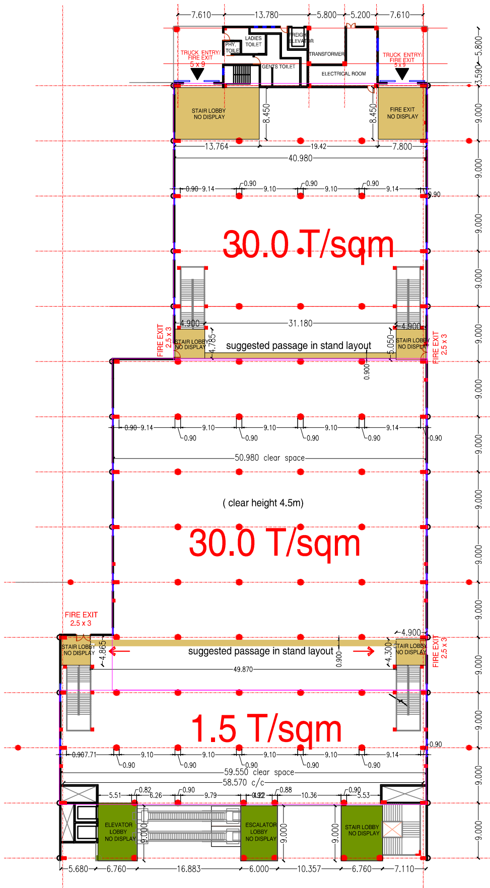
PLAN AT UPPER LEVEL
